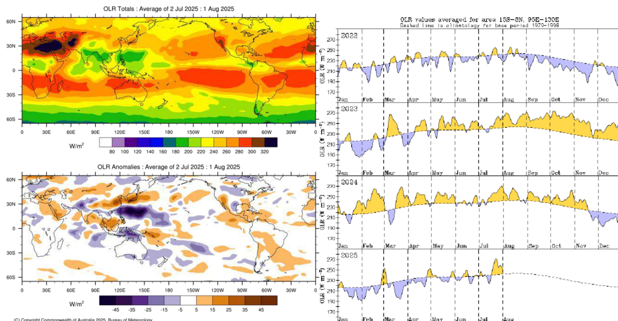
Gambar 2. Grafik OLR ( Outgoing Longwave Radiation )
